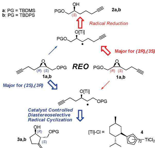
Scheme 1. Concept of Enantioselective Radical Cyclization after Regiodivergent Epoxide Opening (REO)
