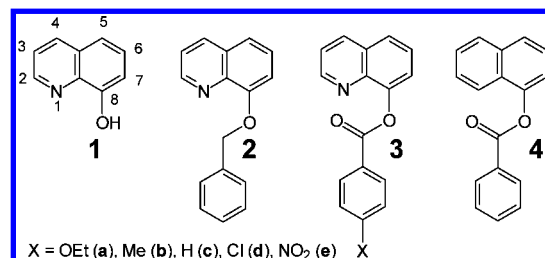
Figure 1. Chemical structure of 8-HQ 1 and its derivatives 2–4 .
