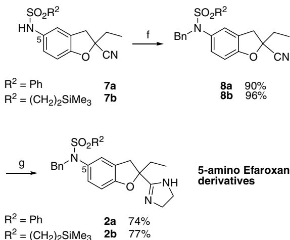
Scheme 4. Reagents and conditions: (f) NaH 1.1 equiv, DMF, 50 °C, BnBr 1.05 equiv, 1 h 30; (g) (1) 0.5 equiv MeONa, MeOH, 21 h, rt; (2) 1.3 equiv ethylenediamine, then 1.3 equiv HCl (1 M in MeOH), 0 °C to rt, 18 h.
