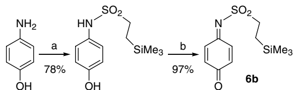
Scheme 1. Reagents and conditions: (a) Me_3Si(CH_2)_2SO_2Cl 1.0 equiv, pyridine/DMF 1:2, 0 °C to rt, then rt for 2 h; (b) Pb(OAc)_4 1 equiv, glacial AcOH, rt, 1 h.
