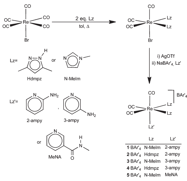
Scheme 1. Synthesis of the “Mixed” Organometallic Compounds [1-5] \cdot \text{BAR}'_4
