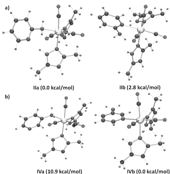
Figure 4. B3LYP/6-31G* optimized structures for cationic complexes 2 (a) and 4 (b).
