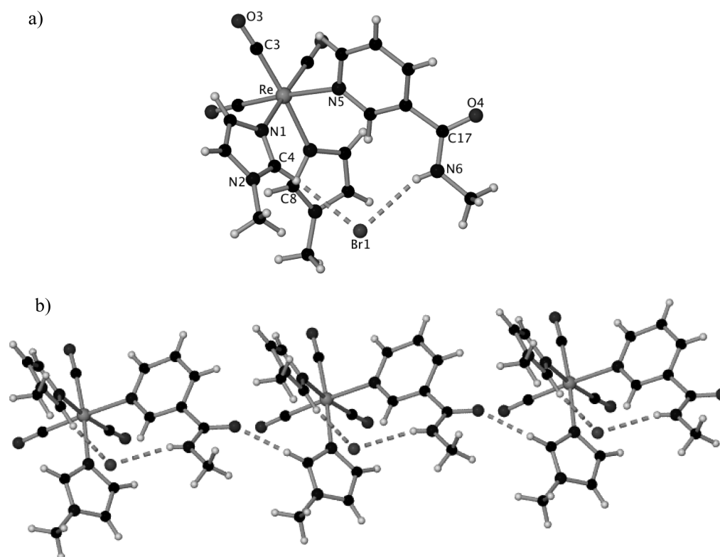
Figure 8. (a) Molecular structure of the 5 \cdot \text{Br} adduct, showing the main intramolecular hydrogen bonds as dashed lines. (b) View of the intermolecular interactions in 5 \cdot \text{Br} , which lead to infinite chains.
