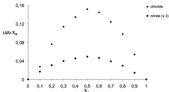
Figure 5. Job plot of receptor 3 · \text{BAR}'_4 toward chloride and nitrate anions.
