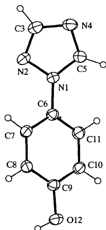
Fig. 1. The molecular structure of (II) showing the atom-numbering scheme. Displacement ellipsoids are drawn at the 30% probability level and H atoms are shown as spheres of an arbitrary radius.
