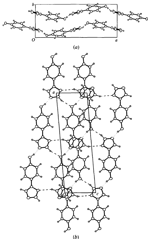
Fig. 2. (a) A projection along the c axis showing the formation of chains in (II) and (b) the packing diagram for (II) along the b axis, illustrating a pair of sheets related by inversion through (\frac{1}{2}, 0, \frac{1}{2}) and the stacking of the triazoles; dotted and dashed lines represent O—H...N and C—H...N/O hydrogen bonds, respectively.
