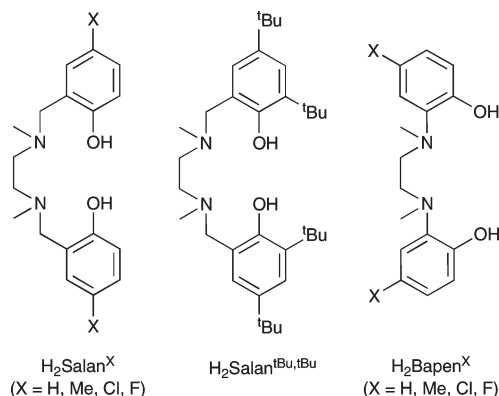
Figure 2. Salan and bapen ligands.
