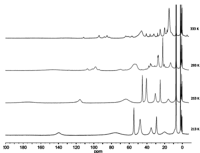
Figure 12. VT 1 H NMR spectra of complex [Fe(bapen F )(Py) 2 ] in d 8 -toluene.
