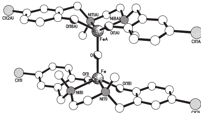
Figure 6. The molecular structure of the C_7 -symmetric complex [\{\text{Fe}(\text{salan}^{\text{Cl}})\}_2(\mu\text{-O})] .
