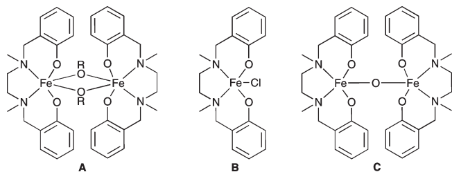
Figure 1. Examples of previously reported iron(III) salan complexes.
