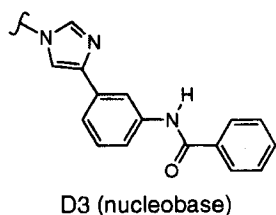
Fig. 7. The selective recognition of T·A and C·G (not shown) base pairs by the nonnatural nucleoside D3 within the pyrimidine·purine·pyrimidine triple-helical binding motif mediated by intercalation of the nucleobase of D3 into double-helical DNA: a) intercalation of the nucleobase of D3 into double-helical DNA within a pyrimidine·purine·pyrimidine triple helix determined by NMR [45]; b) superposition of the nucleobase of L1 with the structure shown in a (view from the top). The upper T·A Watson-Crick base pair has been omitted for clarity. D3 (nucleobase) is shown in green, L1 (nucleobase) is shown in magenta.
