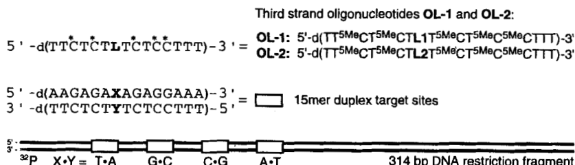
Fig. 4. Sequences of third strand oligonucleotides OL-1 and OL-2 and duplex target sites within a 3'-end- 32 P-labeled 314 base pair (bp) Afl II/Fsp I restriction fragment
