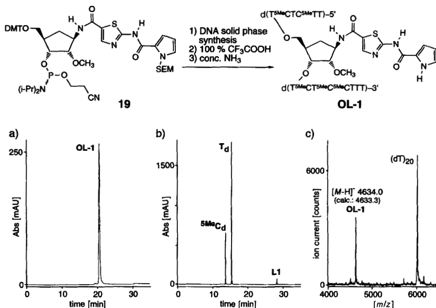
Fig. 3. Synthesis and characterization of oligonucleotide OL-1 : a) HPLC analysis of purified OL-1 (260 nm); b) HPLC analysis of digested OL-1 (snake venom phosphodiesterase and alkaline phosphatase, 260 nm); c) MALDI-TOF-MS analysis of purified OL-1
