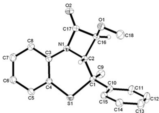
Figure 2. X-ray crystal structure of the racemic major diastereomer \beta -lactam (2S*,2aR*,3R*)- 4c (only one enantiomer is shown) [15]. The atom numbering in the X-ray structure does not follow the IUPAC nomenclature.
