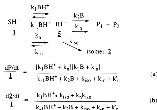
Figure 3. A condensed and simplified version of Figure 2 by which the substrate 1 of Figure 2 is reversibly converted to the phosphorane monoanion 5 with catalysis by the buffer acid \text{BH}^+ or nonbuffer species ( \text{H}^+ , \text{OH}^- , \text{H}_2\text{O} ), and 5 is then converted to isomer 2 or, with catalysis by B or nonbuffer species, to cleavage products \text{P}_1 and \text{P}_2 . The steady-state (in 5 ) equations for cleavage (a) and for isomerization (b) are shown. The constants k_n , k_{-n} , and k'_n include concentrations of such nonbuffer species as \text{OH}^- and \text{H}^+ , so they are functions of pH. The isomerization reaction shows negative catalysis (cf. ref 10) by B , which appears only in the denominator of eq b.
