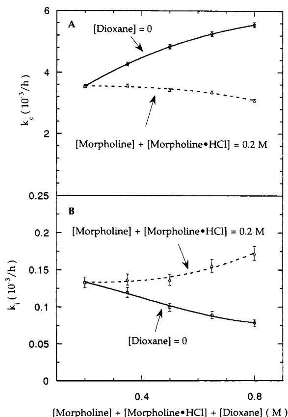
Figure 5. Pseudo-first-order rate constant for (A) the cleavage of 3',5'-UpU and (B) the isomerization of 3',5'-UpU to 2',5'-UpU, both vs the buffer concentration at 60 °C: (○—) 9/1 morpholine/morpholine hydrochloride; (△-- --) 0.2 M morpholine buffer plus an amount of dioxane that brings the total concentration to the amount shown. The ionic strength was maintained at 0.2 M for all runs. The medium effect decreases the rate of the cleavage reaction, but it increases the rate of isomerization, opposite to the effect of the buffer.
