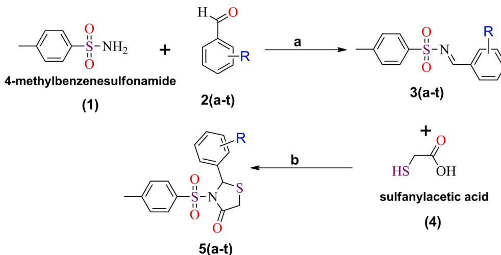
Scheme 1. Scheme for the synthesis of 2-(R-phenyl)-3-[(4-methylphenyl)sulfonyl]-1,3-thiazolidin-4-one derivatives 5 (a-t) . Reagents and Condition: (a) C_2H_5OH , reflux, 80^\circ C , 5–6 h.; (b) DCC ( N,N -dicyclohexylcarbodiimide), C_2H_5OH , reflux 120^\circ C , 9–10 h.
