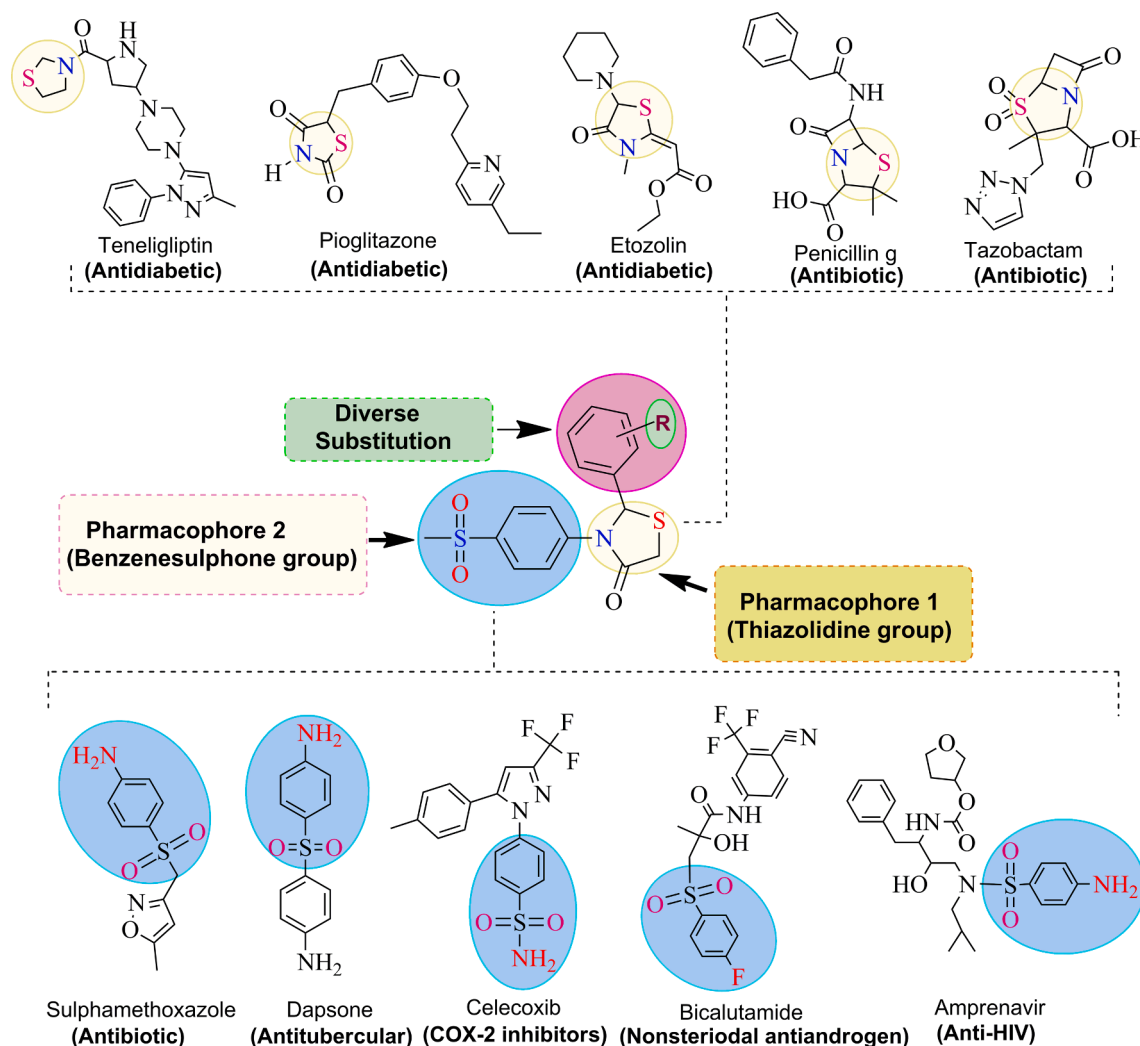
Fig. 1. Chemical structures of commercially available drugs containing Thiazolidine and benzenesulphone moieties.
