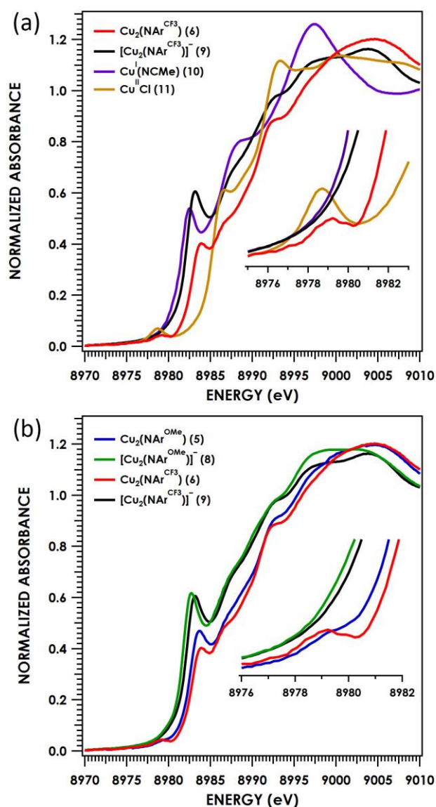
Figure 5. Cu K-edge XAS spectra of (a) [(^t\text{Bu}^{\text{dmx}})\text{Cu}_2(\mu^2\text{-NAr})]^n for n = 0 , Ar: 3,5-(CF 3 ) 2 -C 6 H 3 ( 6 , red); n = -1 , Ar: 3,5-(F 3 C) 2 C 6 H 3 ( 9 , black); and mononuclear (^t\text{Bu}^{\text{L}})\text{Cu}^{\text{I}}(\text{NCMe}) ( 10 , purple); (^t\text{Bu}^{\text{L}})\text{Cu}^{\text{I}}\text{Cl} ( 11 , gold); (b) n = 0 , Ar: 4-MeOC 6 H 4 ( 5 , blue); Ar: 3,5-(F 3 C) 2 C 6 H 3 ( 6 , red); n = -1 , Ar: 4-MeOC 6 H 4 ( 8 , green); Ar: 3,5-(F 3 C) 2 C 6 H 3 ( 9 , black).
