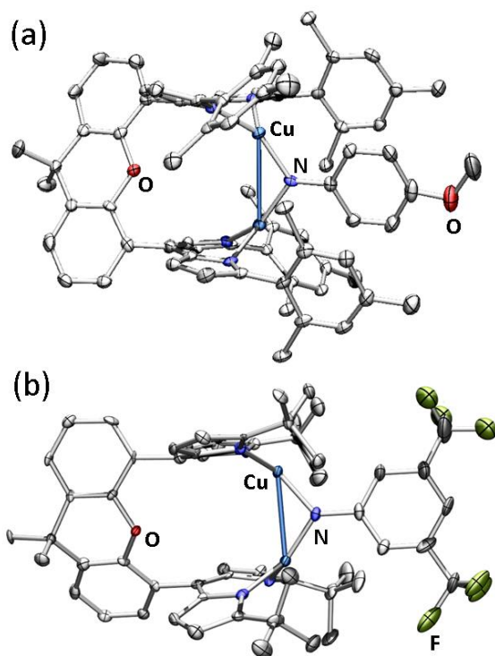
Figure 2. Solid state molecular structures of (a) (Mes-dmx)Cu 2 (μ 2 -N(C 6 H 4 OMe)) ( 2 ), (b) (tBu-dmx)Cu 2 (μ 2 -N(3,5-(F 3 C) 2 C 6 H 3 )) ( 6 ) at 50 % ellipsoid probability. Color scheme: Cu (cobalt blue), F (yellow-green), N (blue), O (red). Solvent molecules, solid-state disorder, and hydrogen atoms are omitted for clarity.
