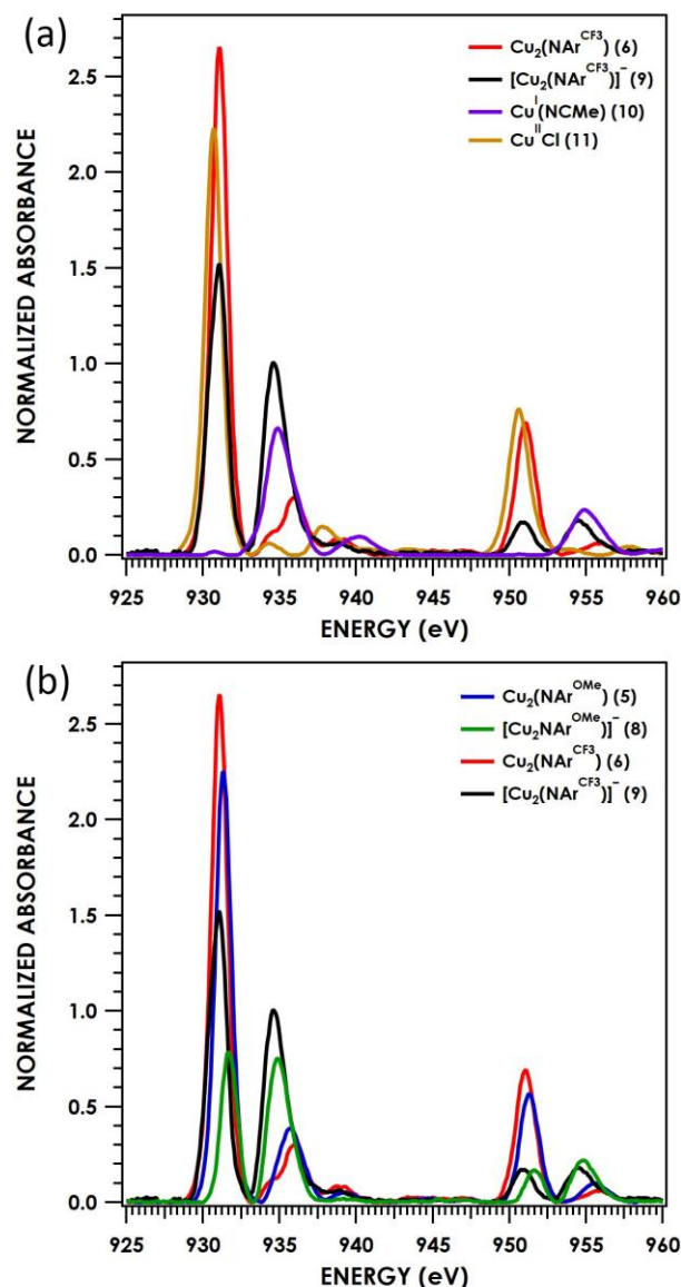
Figure 6. Cu L 2,3 -edge XAS spectra of (a) [(t\text{Bu-dmx})\text{Cu}_2(\mu^2\text{-NAr})]^n for n = 0 , Ar: 3,5-(CF 3 ) 2 -C 6 H 3 ( 6 , red); n = -1 , Ar: 3,5-(F 3 C) 2 C 6 H 3 ( 9 , black); and mononuclear (t\text{BuL})\text{Cu}^{\text{I}}(\text{NCMe}) ( 10 , purple); (t\text{BuL})\text{Cu}^{\text{II}}\text{Cl} ( 11 , gold); (b) n = 0 , Ar: 4-MeOC 6 H 4 ( 5 , blue); Ar: 3,5-(F 3 C) 2 C 6 H 3 ( 6 , red); n = -1 , Ar: 4-MeOC 6 H 4 ( 8 , green); Ar: 3,5-(F 3 C) 2 C 6 H 3 ( 9 , black).
