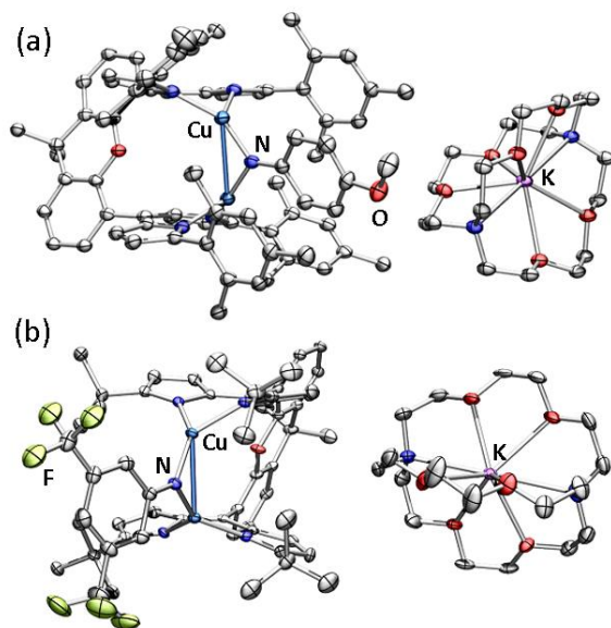
Figure 3. Solid state molecular structures of (a) [K(C 222 )][( Mes dmx)Cu 2 (μ 2 -N(C 6 H 4 OMe))] ( 7 ) at 35 % ellipsoid probability and (b) [K(C 222 )][( tBu dmx)Cu 2 (μ 2 -N(3,5-(F 3 C) 2 C 6 H 3 ))] ( 9 ) at 50 % ellipsoid probability. Color scheme: Cu (cobalt blue), F (yellow-green), N (blue), O (red), K (pink). Solvent molecules, solid-state disorder, and hydrogen atoms are omitted for clarity.
