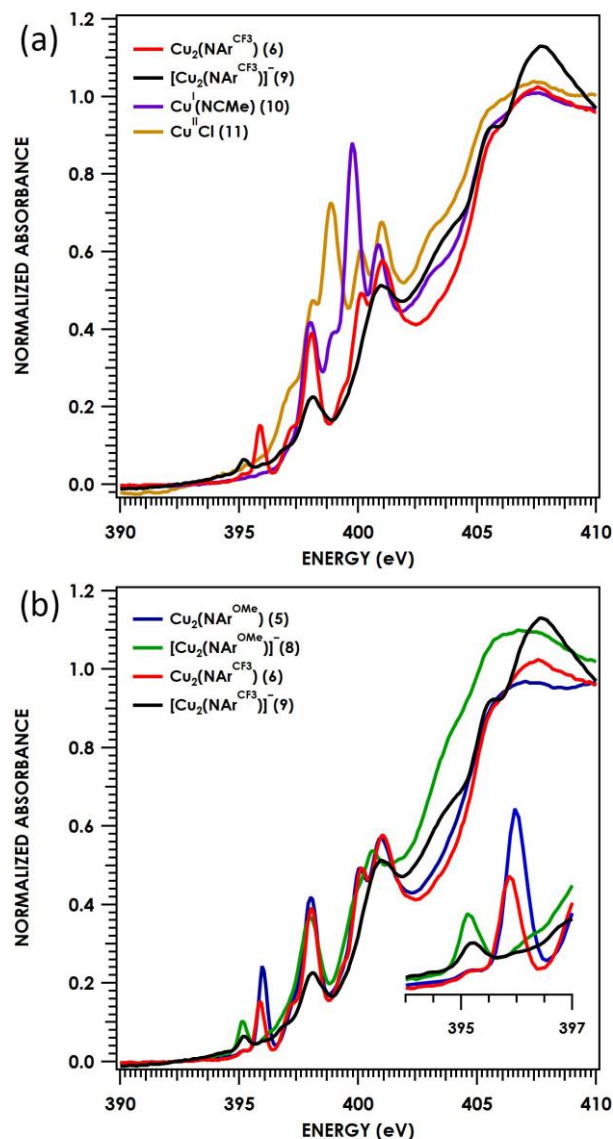
Figure 7. N K-edge XAS spectra of (a) [(t\text{Bu-dmx})\text{Cu}_2(\mu^2\text{-NAr})]^n for n = 0 , Ar: 3,5-(CF 3 ) 2 -C 6 H 3 ( 6 , red); n = -1 , Ar: 3,5-(F 3 C) 2 C 6 H 3 ( 9 , black); and mononuclear (t\text{BuL})\text{Cu}^{\text{I}}(\text{NCMe}) ( 10 , purple); (t\text{BuL})\text{Cu}^{\text{II}}\text{Cl} ( 11 , gold); (b) n = 0 , Ar: 4-MeOC 6 H 4 ( 5 , blue); Ar: 3,5-(F 3 C) 2 C 6 H 3 ( 6 , red); n = -1 , Ar: 4-MeOC 6 H 4 ( 8 , green); Ar: 3,5-(F 3 C) 2 C 6 H 3 ( 9 , black).
