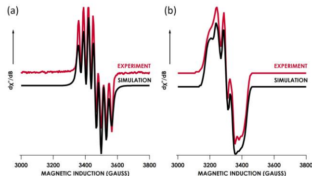
Figure 4. (a) Solution 2-methyltetrahydrofuran (9.843 GHz) EPR spectrum of 7 obtained at 298 K expanded to show an isotropic S = 1/2 signal (red) simulated (black) with the following parameters: g iso = 2.033, σ gx = 0.0277, σ gy = 0.0039, σ gz = 0.0051; 63 Cu A iso = 87.4 MHz; 14 N A iso = 17.8 MHz. (b) Frozen 2-methyltetrahydrofuran (9.378 GHz) EPR spectrum 7 obtained at 4 K expanded to show an anisotropic S = 1/2 signal (red) simulated (black) with the following parameters: g x = 1.979, g y = 2.032, g z = 2.074; σ gx = 0.0080, σ gy = 0.0014, σ gz = 0.0098; 63 Cu A x = 9.3 MHz, A y = 43.9 MHz, A z = 9.7 MHz; 14 N A x = 86.6 MHz, A y = 125.6 MHz, A z = 130.3 MHz.
