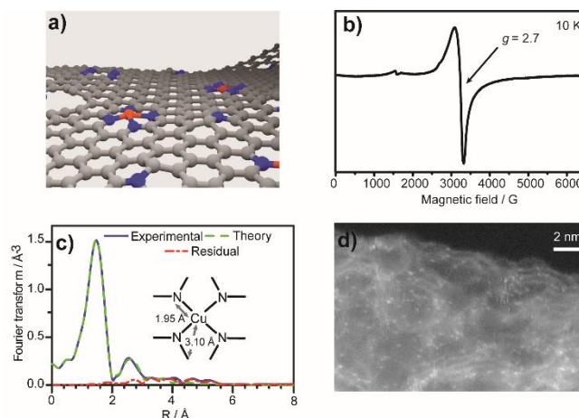
Figure 1. Structural and morphological characterization of Cu 0.5 NC. (a) Schematic representation; (b) EPR spectrum recorded at 10 K of Cu 0.5 NC diluted in an amorphous silica matrix; (c) Cu K-edge EXAFS analysis in the Fourier-transformed space; (d) HAADF-STEM image.
