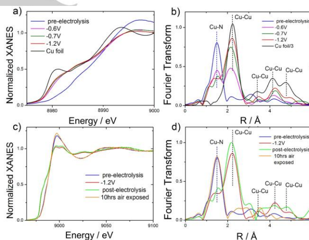
Figure 3. Operando XAS characterization of Cu 0.5 NC at the Cu-K edge. (a) K-edge XANES spectra of Cu 0.5 NC under no potential applied (blue line), Cu 0.5 NC during electrolysis at -0.6 V vs. RHE (pink line), at -0.7 V vs. RHE (green line), at -1.2 V vs. RHE (red line) and metallic copper (black line), (b) Fourier transform of the experimental EXAFS spectra of Cu 0.5 NC no potential applied (blue line), Cu 0.5 NC during electrolysis at -0.6 V vs. RHE (pink line), at -0.7 V vs. RHE (green line), at -1.2 V vs. RHE (red line) and metallic copper (black line), (c) Comparison between the K-edge XANES experimental spectrum of Cu 0.5 NC under no potential applied (blue line), Cu 0.5 NC during electrolysis at -1.2 V vs. RHE (red line), after electrolysis under no potential applied (green line) and Cu 0.5 NC after electrolysis at -1.2 V vs. RHE then sample exposed to air for 10 hours (orange line) (d) Fourier transform of the experimental EXAFS spectra of Cu 0.5 NC under no potential applied (blue line), Cu 0.5 NC during electrolysis at -1.2 V vs. RHE (red line), after electrolysis under no potential applied (green line) and Cu 0.5 NC after electrolysis at -1.2 V vs. RHE then sample exposed to air for 10 hours (orange line).
