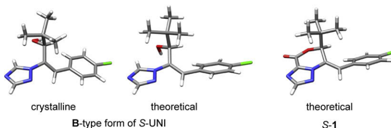
Figure 4. 3D structures of S-UNI (crystalline and theoretical) and S-1 (theoretical).
