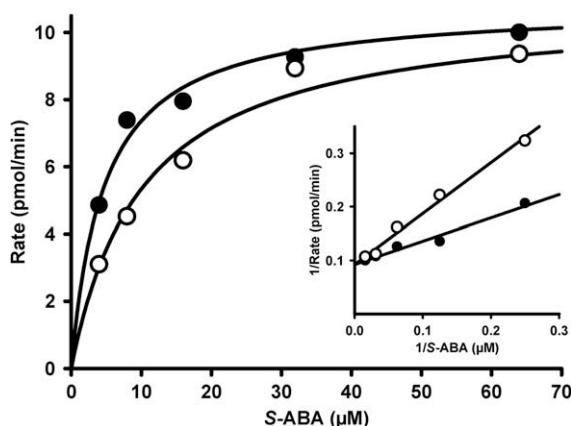
Figure 5. Competitive inhibition of ABA 8'-hydroxylase by 3R- 5 . Assays contained S-ABA (●) or S-ABA and 0.5 \mu M 3R- 5 (○). The inset is a double-reciprocal plot for the same data. The same mode of inhibition was observed for 3S- 5 and S- and R- 9 (data not shown).
