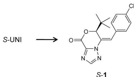
Scheme 1. Synthesis of S-1 . Reagents and conditions: \text{ClCOOCCl}_3 , pyridine, dry \text{CH}_2\text{Cl}_2 , 0^\circ\text{C} , 98%. R-1 and racemic 1 were synthesized by the same scheme from R-UNI and racemic UNI , respectively.
