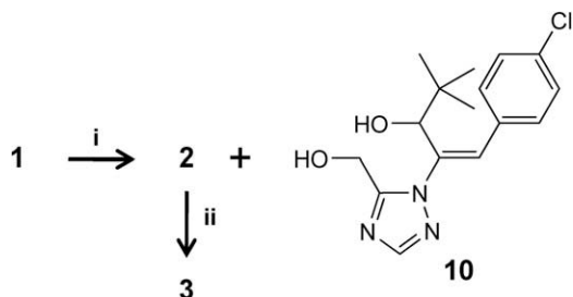
Scheme 2. Synthesis of 2 and 3 . Reagents and conditions: (i) \text{LiAlH}_4 , dry \text{Et}_2\text{O} , 0^\circ\text{C} , 47% ( 2 ); (ii) \text{Et}_3\text{SiH} , \text{BF}_3\cdot\text{Et}_2\text{O} , rt, 13%.
