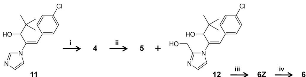
Scheme 3. Synthesis of 4 , 5 , and 6 . Reagents and conditions: (i) \text{ClCOOCCl}_3 , pyridine, dry \text{CH}_2\text{Cl}_2 , 0^\circ\text{C} , 94%; (ii) \text{LiAlH}_4 , dry \text{Et}_2\text{O} , 0^\circ\text{C} , 38% ( 5 ), 24% ( 18 ); (iii) \text{ZnCl}_2 , dry 1,2-dichloroethane, 100^\circ\text{C} , 51%; (iv) UV 365 nm, \text{EtOAc} , rt, 32%.
