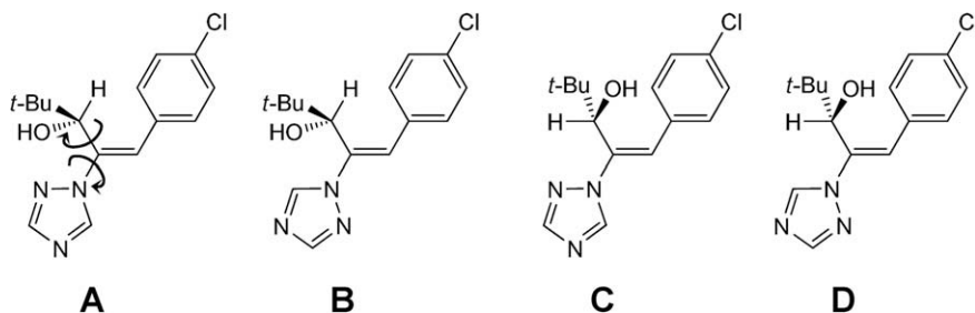
Figure 2. Four conformers A–D generated by bond rotations of C2–N1'' and C2–C3 in UNI.
