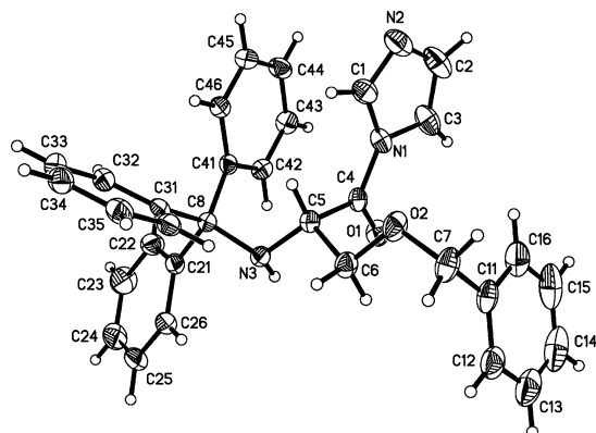
Figure 1. Solid-state structure of acid imidazolidine 8 .
