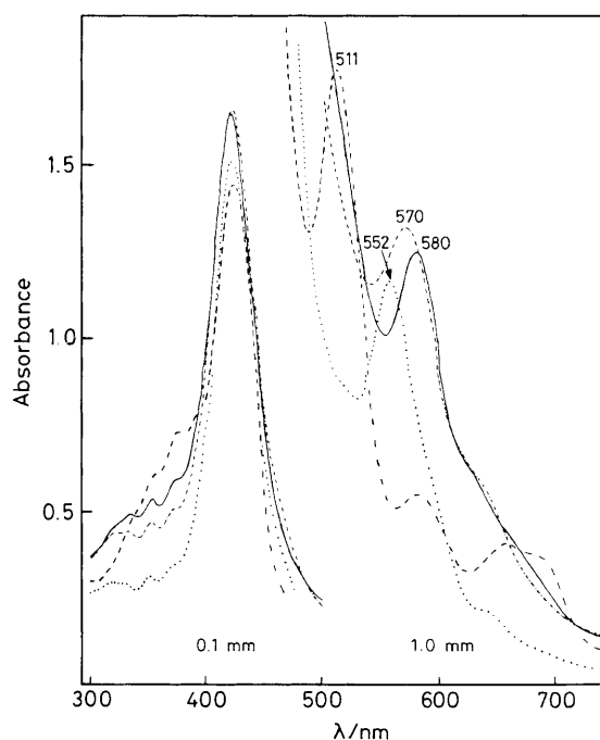
Figure 1. Optical spectra of 5,10,15-trianthracenyl-20-(4-methoxyphenyl)porphyrinatoiron(III) complexes in \text{CH}_2\text{Cl}_2 . Compound (1) (—), (2) (---), (3) (·····), and (4) (-·-·-). [(1)], [(3)] = 0.90 mm; [(2)], [(4)] = 0.99 mm. The optical path lengths are indicated.
