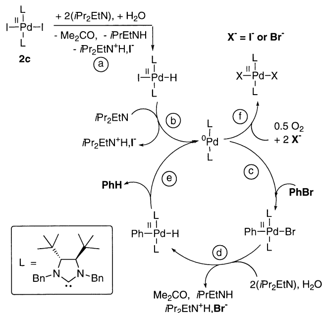
Scheme 8. Reduction of 2c by i Pr 2 EtN in the presence of PhBr.
