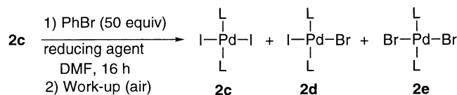
Scheme 9. Reduction of 2c in the presence of PhBr.
