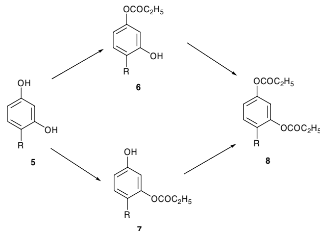
Scheme 2. CAL-B-catalyzed regioselective acylation of 4-substituted resorcinols ( 5 ). R: a, Me; b, Et; c, (CH 3 ) 3 CCH 2 C(CH 3 ) 2 –; d, Bn; e, Cl; f, Br.
