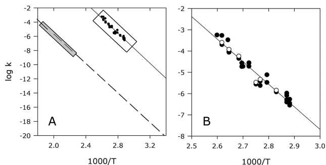
Figure 1. Arrhenius plots showing the hydrolysis of \text{NP}^{2-} in cyclohexane. Observed first-order rate constants ( k ) are not corrected for water concentration. For comparison, the rates of reaction in water are shown as a broken line with the temperature range over which data were collected indicated by the gray box (A). Data obtained by NMR are shown as solid points, and data collected by the molybdate assay for inorganic phosphate are shown as open points (B). In A, the vertical axis on the right corresponds to 25 °C.
