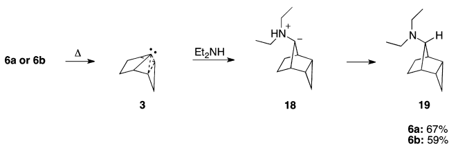
Scheme 6. Thermolysis of Oxadiazolines 6a and 6b in the Presence of Diethylamine
