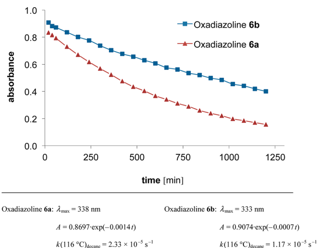
Figure 3. Decay of oxadiazolines 6a and 6b at 116 °C monitored using their UV absorbance maxima and found to be first-order.
