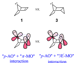
Figure 1. Interaction of the single bond Walsh orbital in carbene 3 mimics that of the double bond \pi -MO in carbene 1 , thereby establishing a two-electron, three-center bond with each carbene's p-AO.
