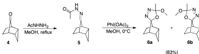
Scheme 2. Synthesis of the Oxadiazoline ( 6 ) Used To Generate Carbene 3
