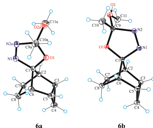
Figure 2. Single-crystal X-ray diffraction was used to elucidate the structures of the rel -(1' R ,2' r ,2' R ,4' S ,5' S ,5' S )-5-methoxy-5-methylspiro[2,5-dihydro-1,3,4-oxadiazole-2,8'-tricyclo[3.2.1.0 2,4 ]octane] ( 6a ) and rel -(1' R ,2' s ,2' R ,4' S ,5' S ,5' S )-5-methoxy-5-methylspiro[2,5-dihydro-1,3,4-oxadiazole-2,8'-tricyclo[3.2.1.0 2,4 ]octane] ( 6b ).
