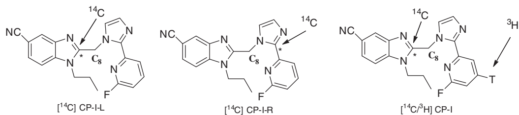
Figure 2. Positions of C-14 and H-3 labels.
