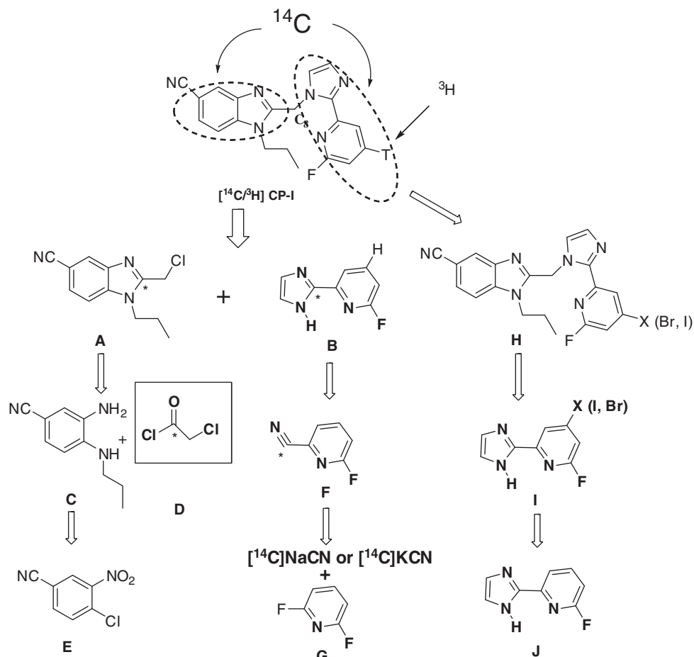
Figure 3. Retro-synthetic pathway of [ 14 C]CP-I and [ 3 H]CP-I.
