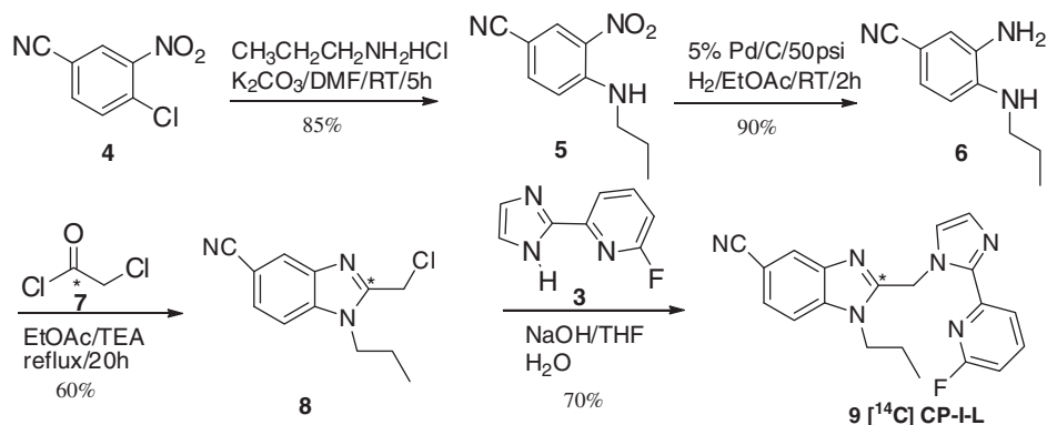
Scheme 1. Synthesis of [ 14 C]CP-I-L.
