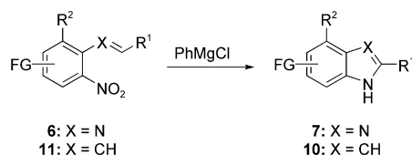
Scheme 4. Preparation of functionalized benzimidazoles and indoles.
