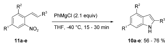
Scheme 10. Preparation of functionalized indoles 10a–e by treatment of nitro-substituted stilbenes 11a–e with phenylmagnesium chloride.
