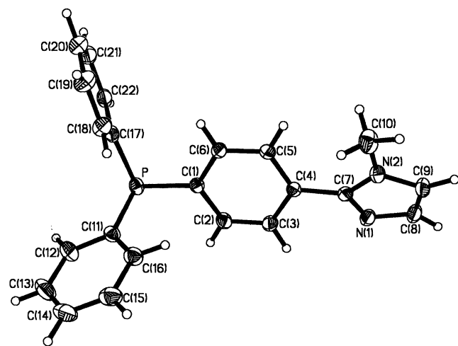
Fig. 1. A perspective drawing of 4 with 20% probability thermal ellipsoids for the non-hydrogen atoms
