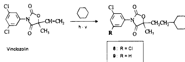
Figure 5. Photodegradation of vinclozolin in the presence of cyclohexane.
