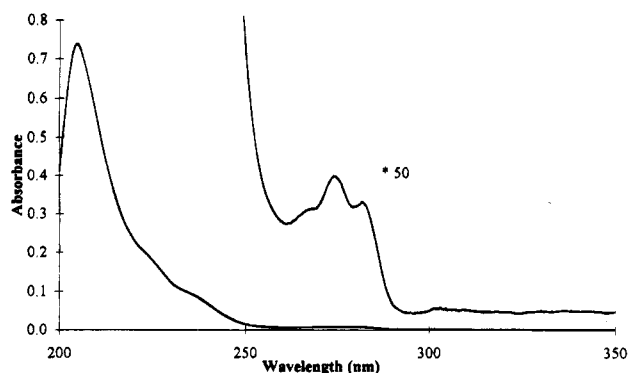
Figure 2. UV absorption spectrum of vinclozolin in 2-propanol.
