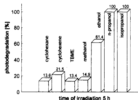
Figure 3. Photodegradation (λ > 280 nm) of vinclozolin after 5 h of irradiation in various organic solvents (50 mg/50 mL).
