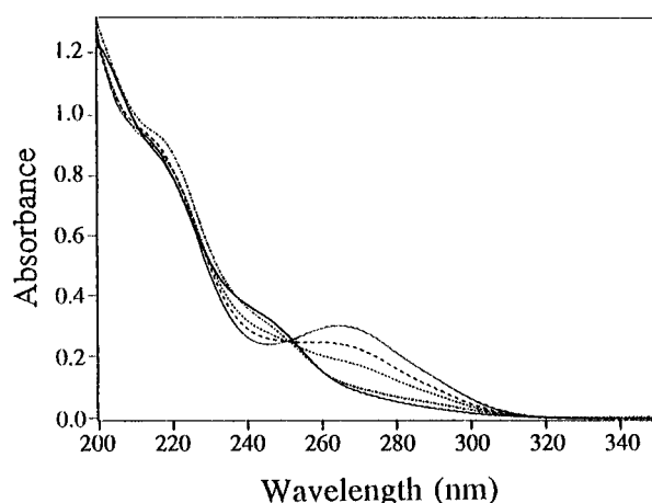
Figure 2. Protonation of [\text{ReO}_2(1\text{-MeIm})_4]\text{I} ( 3.30 \times 10^{-5}\text{ M} ) with \text{HBF}_4 in methanol. \text{H}^+/\text{Re} ratio (from top to bottom at 270 nm): 0, 0.12, 0.23, 0.70, 1.10.
