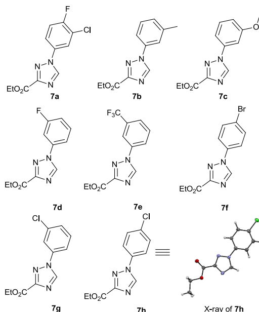
Figure 1: Representative [1,2,4]-triazoles prepared in flow.
