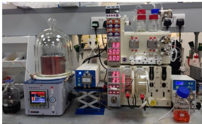
Figure 2: Flow reactor used for the synthesis of pyrrolo[1,2- c ]pyrimidine.
