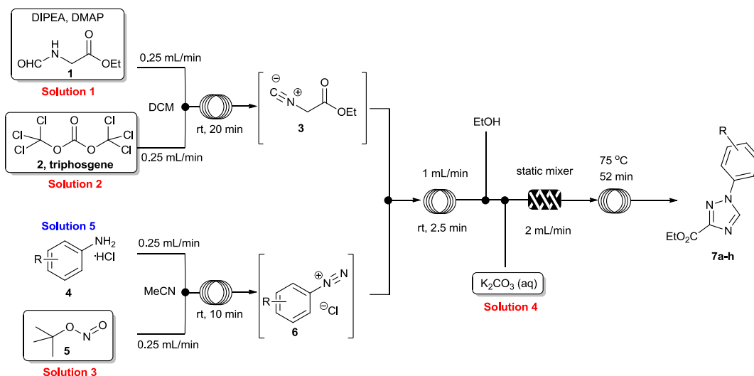
Scheme 3: Multi-step flow approach towards 1,2,4-triazoles.
