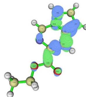
Figure 3. Dual descriptor Fukui function of pyrrolo[1,2- c ]pyrimidine ( 11 ). (green electrophilic regions; blue nucleophilic regions)
