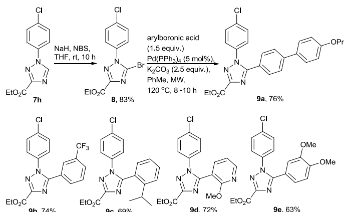
Scheme 4: Functionalization study of triazole 7h .
