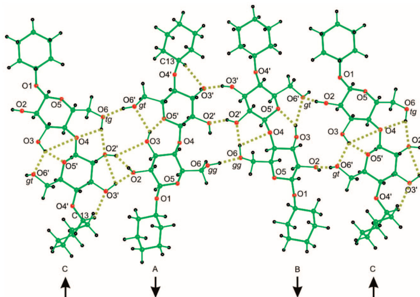
Figure 9. Four molecules of 8 in the (210) plane, in which all neighboring molecules are hydrogen bonded to each other. The second C molecule is shown so that the B–C hydrogen bonds are included. The S and T molecules are not shown, nor are E and F. Intramolecular hydrogen bonds are repetitions from Figure 7.
