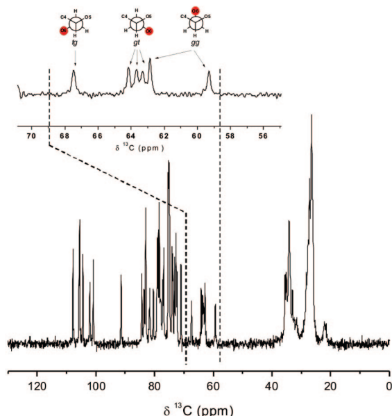
Figure 7. Solid-state ( ^{13}\text{C} CPMAS, CP = 1 ms, 150.9 MHz) NMR of compound 8 . Inset: C-6 region showing all three preferred conformations, gt/gg/tg = 3:2:1 .
