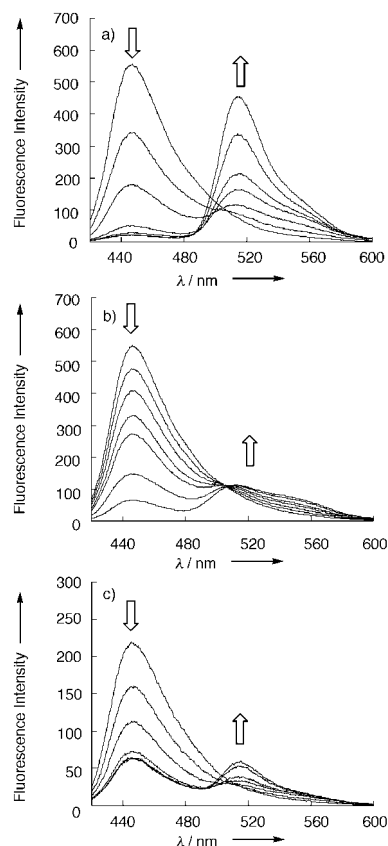
Figure 3. The emission spectra of compounds 1–3 ( 1.0\ \mu\text{M} ) after the addition of PTP1B ( 10\ \mu\text{g mL}^{-1} ) in 0.1\text{M} HEPES buffer (pH 7.4) containing 1.0\text{ mM} DTT and EDTA at 30^\circ\text{C} . a) Emission spectra of 1 measured at 1, 5, 10, 20, 30, 60, and 120 min after the addition, \lambda_{\text{ex}} = 402\text{ nm} . b) Emission spectra of 2 measured at 1, 5, 10, 20, 30, 60, and 180 min after the addition, \lambda_{\text{ex}} = 402\text{ nm} . c) Emission spectra of 3 measured at 1, 5, 10, 30, 60, 120, and 180 min after the addition, \lambda_{\text{ex}} = 407\text{ nm} .
