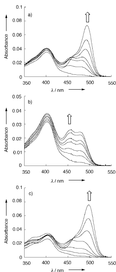
Figure 4. The absorption spectra of compounds 1–3 ( 1.0\ \mu\text{M} ) after the addition of PTP1B ( 10\ \mu\text{g mL}^{-1} ) in 0.1\text{M} HEPES buffer (pH 7.4) containing 1.0\text{ mM} DTT and EDTA at 30^\circ\text{C} . a) Absorption spectra of 1 measured at 1, 5, 10, 20, 45, 60, and 120 min after the addition. b) Absorption spectra of 2 measured at 1, 5, 10, 20, 30, 60, and 120 min after the addition. c) Absorption spectra of 3 measured at 1, 5, 10, 20, 120, 240, and 360 min after the addition.
