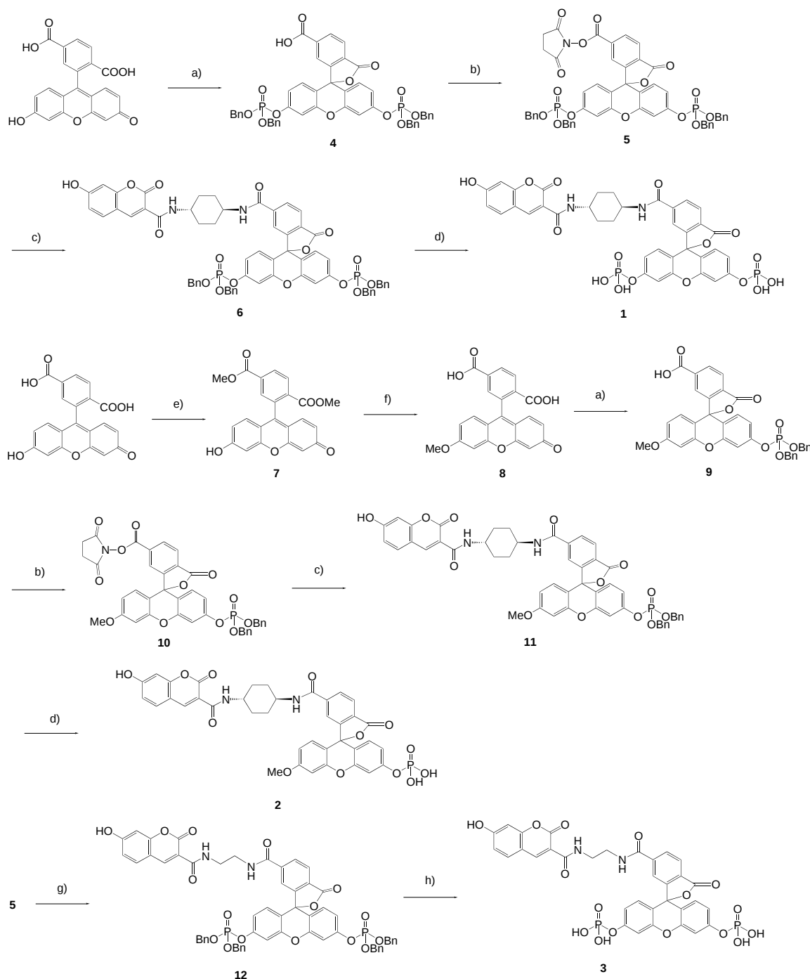
Scheme 2. Synthesis of compounds 1–3 : a) (\text{BnO})_2\text{PN}(\text{iPr})_2 , 1 H -tetrazole, \text{NEt}_3 , m CPBA, \text{CHCl}_3 ; b) N -hydroxysuccinimide, EDC·HCl, \text{CHCl}_3 ; c) 7-hydroxycoumarin-3-carboxylic succinimidyl ester, trans -1,4-cyclohexanediamine, DMF; d) Pd/C, \text{H}_2 , MeOH; e) \text{H}_2\text{SO}_4 , MeOH; f) \text{CH}_3\text{I} , \text{Cs}_2\text{CO}_3 , DMF, aq NaOH; g) 7-hydroxycoumarin-3-carboxylic succinimidyl ester, ethylenediamine, DMF; h) Pd/C, \text{H}_2 , MeOH/ \text{CHCl}_3 .
