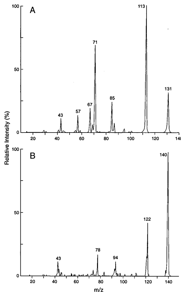
Figure 3. API-MS/MS daughter ion spectra of the 131 u (A) and 140 u (B) ion peaks attributed to the [M + H]^+ ions of HC(O)CH_2CH(OH)CH_2CH_2CHO and DC(O)CD_2CD(OH)CD_2CD_2CDO (after -OD to -OH exchange), respectively.
