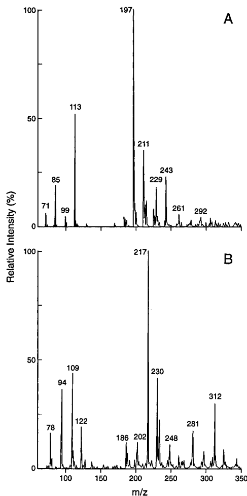
Figure 1. API-MS spectra of irradiated \text{CH}_3\text{ONO} –NO–cyclohexane–air (A) and \text{CH}_3\text{ONO} –NO–cyclohexane- d_{12} –air (B) mixtures.
