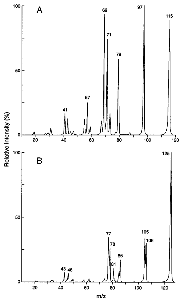
Figure 4. API-MS/MS daughter ion spectra of the 115 u (A) and 125 u (B) ion peaks attributed to the [M + H]^+ ions of \text{HC(O)CH}_2\text{CH}_2\text{CH}_2\text{CH}_2\text{CHO} and \text{DC(O)CD}_2\text{CD}_2\text{CD}_2\text{CD}_2\text{CDO} , respectively.
