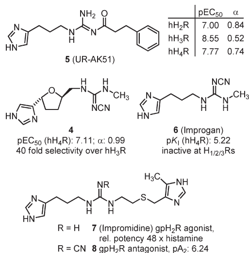
Figure 2. Imidazolylalkylguanidine derivatives reported as histamine receptor ligands.
