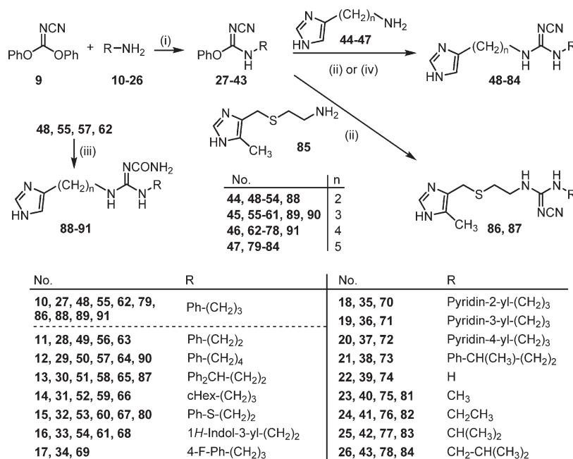
Scheme 1. Synthesis of the Isoorea Precursors 27–43 , the Cyanoguanidines 48–84 , 86 , and 87 , and the Carbamoylguanidines 88–91 a
