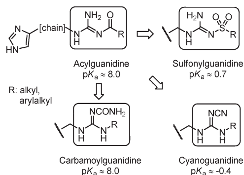
Figure 3. Replacement of the central acylguanidine group with a nonbasic cyanoguanidine or sulfonylguanidine group and a basic carbamoylguanidine group.
