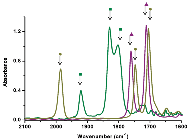
Figure 1. Overlaid IR spectra of 1 [■, green: \nu(\text{NO}) 1932 (s), 1831 (s), 1804 (vs) \text{cm}^{-1} ], 2 [●, olive: \nu(\text{CO}) 1986 (s); \nu(\text{NO}) 1744 (s), 1702 (vs) \text{cm}^{-1} ], and 3 [▲, purple: \nu(\text{NO}) 1763 (s), 1715 (vs) \text{cm}^{-1} ] in THF solution.
