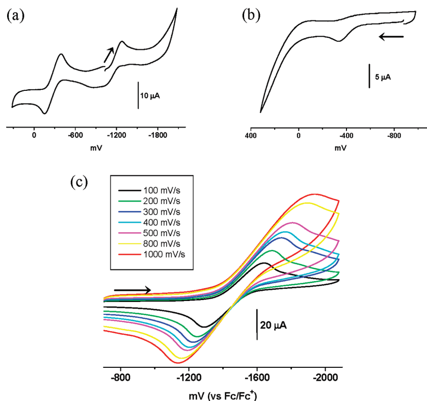
Figure 2. Cyclic voltammograms of (a) 1 and (b) 2 at scan rates of 200 and 100 \text{mV/s} , respectively, and (c) 3 at scan rates of 100–1000 \text{mV/s} in 2 mM THF solution.
