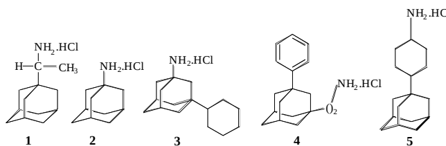
Figure 1. Structures of trypanocidal aminoadamantanes [4]. The concentrations that inhibited growth of bloodstream form T. brucei by 50% (IC 50 ) were established as follows: (1) 7.04 \mu M; (2) > 132 \mu M; (3) 0.52 \mu M; (4) 0.62 \mu M; (5) 0.33 \mu M.
