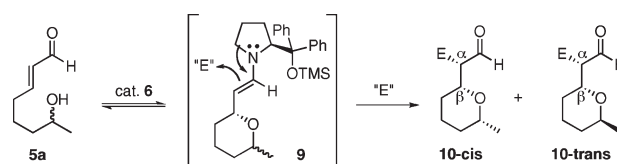
Scheme 2. Cascade by Enamine-Catalyzed Intermolecular Reaction
