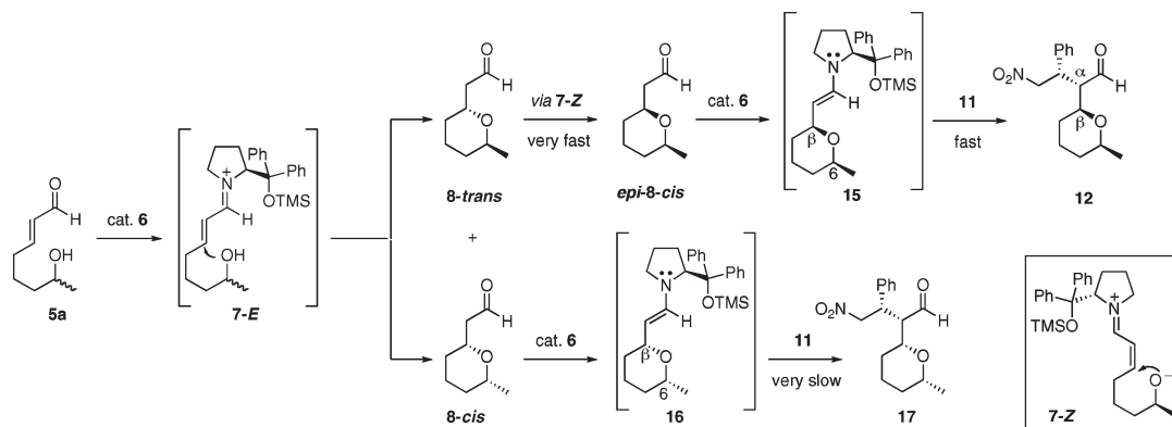
Scheme 4. Proposed Mechanism of Organocascade Kinetic Resolution
