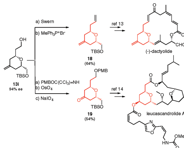
Scheme 5. Synthetic Utility of Resolved Oxa-Michael Adducts
