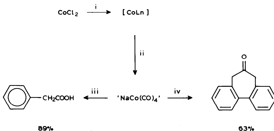
Scheme 2. Reagents and conditions: (i) \text{NaBH}_4/\text{C}_2\text{H}_5\text{OH} , CO, 15 min, 0^\circ\text{C} , (ii) 5 N NaOH (10 ml)/CO/room temperature 10 min. (iii) Benzyl bromide, benzyl triethylammonium bromide, CO, 50^\circ\text{C} , 2 h, (iv) 2,2'-bis(bromomethyl)biphenyl, benzyl triethylammonium bromide, CO, 50^\circ\text{C} , 2 h.
