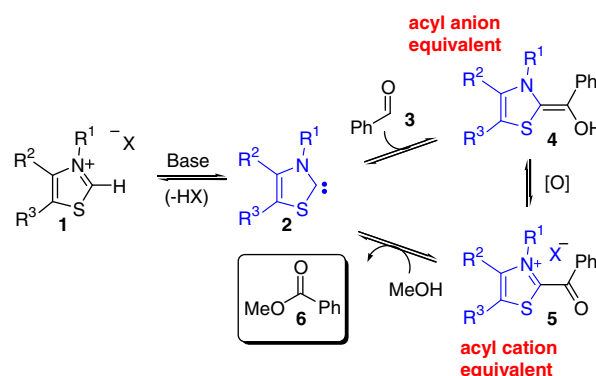
Scheme 1. Proposed mechanism of nucleophilic carbene-catalysed aldehyde esterification.
