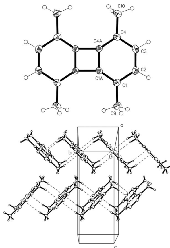
Figure 5. Top: The molecule of compound 8 in the crystal. Ellipsoids represent 50 % probability levels. Only the asymmetric unit is numbered. Selected bond lengths (Å) and angles ( ^\circ ): C1–C1A 1.372(2) , C1–C2 1.424(2) , C2–C3 1.384(2) , C3–C4 1.425(2) , C4–C4A 1.375(2) , C1A–C4A 1.424(2) , C1A–C4A#1 1.523(2) ; C4–C4A–C1A#1 146.9(1) , C1–C1A–C4A#1 146.4(1) . Symmetry operator #1: -x, 1-y, 1-z . Bottom: packing diagram of compound 8 ; dashed lines indicate C–H... \pi interactions.
