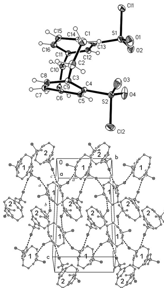
Figure 10. Top: one of the two independent molecules of compound 26 in the crystal. Ellipsoids represent 30% probability levels. Bottom: packing diagram of compound 26 . Boldface numerals indicate independent molecules 1 and 2. Dashed lines and italic letters (the latter indicate the contacts formed by one molecule, see text) indicate Cl⋯O interactions. H atoms are omitted.
