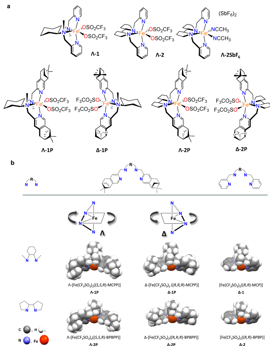
Figure 1. Catalyst structure: (a) 3D chemical diagrams of Λ-1 , Λ-2 , Λ-2SbF 6 , Λ-1P , Δ-1P , Λ-2P , and Δ-2P ; (b) space-filling diagrams of Λ-1P , Δ-1P , Λ-2P , Δ-2P , \Delta -[Fe(CF 3 SO 3 ) 2 [( R,R,R )-MCPP]] ( Δ-1 ) 57 and Δ-2 . 58 Counterions and solvent of crystallization have been omitted for clarity. Details on the experimental parameters of the X-ray diffraction analysis and tables with bond distances and angles are given in the Supporting Information.
