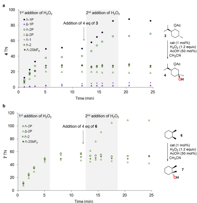
Figure 2. Catalyst stability: (a) oxidation of (–)-menthyl acetate ( 3 ) (formation of 4 in the hydroxylation of 3 represented versus time in two-step addition of \text{H}_2\text{O}_2 in presence of large excess of substrate); (b) oxidation of cis -1,2-dimethylcyclohexane ( 6 ) (formation of 7 in the hydroxylation of 6 represented versus time in two-step addition of \text{H}_2\text{O}_2 in the presence of a large excess of substrate).
