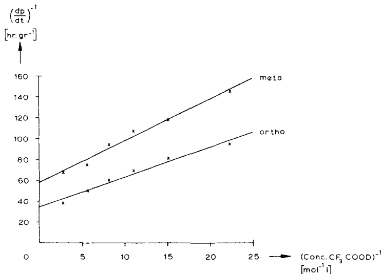
Fig. 3. Photodeuteration of anisole with CF_3COOD in tetrahydrofuran
