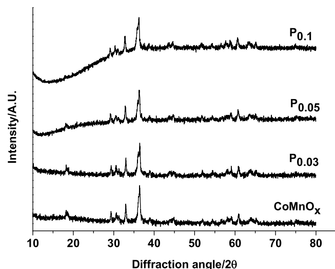
Fig. 1. XRD pattern of P doped catalysts.
