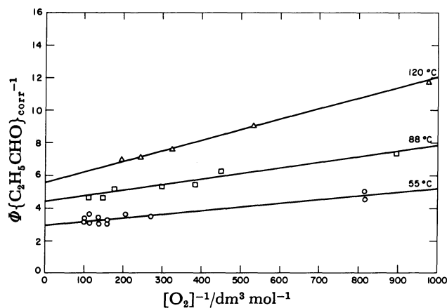
Fig. 9. Plots of \Phi\{C_2H_5CHO\}_{\text{corr}}^{-1} , computed using values of k_6/k_2 in Table 7, vs. [O_2]^{-1} at 55, 88, and 120 °C. The plots at 88 and 120 °C are displaced upward by 2 and 3 units, respectively, for clarity.
