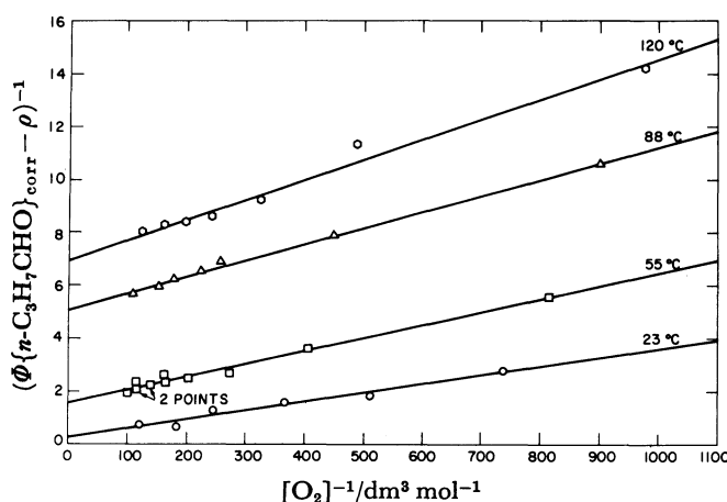
Fig. 6. Plots of (\Phi\{n-C_3H_7CHO\}_{corr}-\rho)^{-1} , computed using values of k_6/k_2 in Table 7, vs. [O_2]^{-1} . The plots are displaced upwards by 5, 3, -1, and -2 units, respectively, for 120, 88, 55, and 23^\circ\text{C} for clarity.
