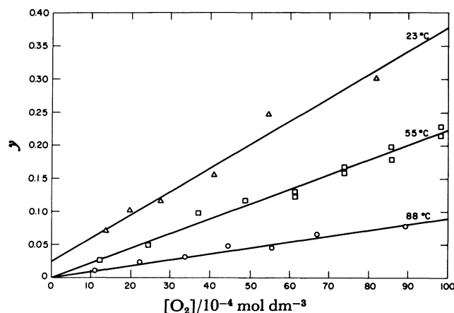
Fig. 7. Plots of y =left-hand side of Eq. e as computed using values of k_{13a}/k_{13} and k_{13a}/k_{12} in Table 7, vs. [O_2] . The plot at 23^\circ\text{C} is displaced upward by 0.025 unit for clarity.
