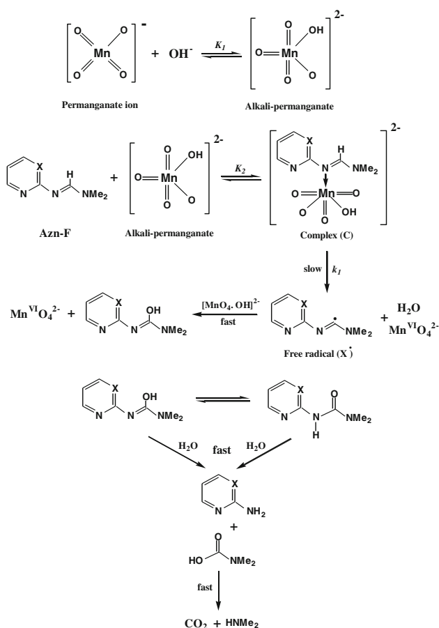
Scheme 2 Mechanism of oxidation of azinyl formamidines by alkaline permanganate
