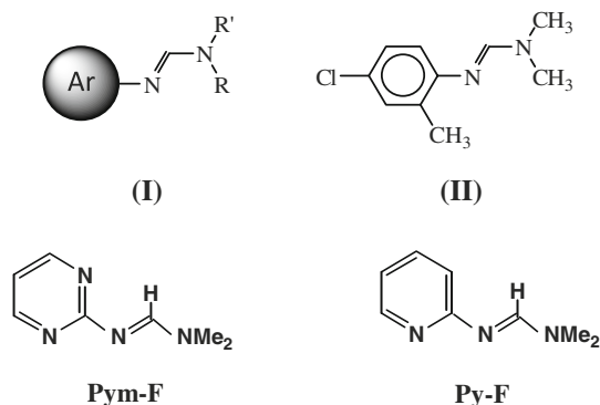
Scheme 1 Structure of some azinyl formamidines
