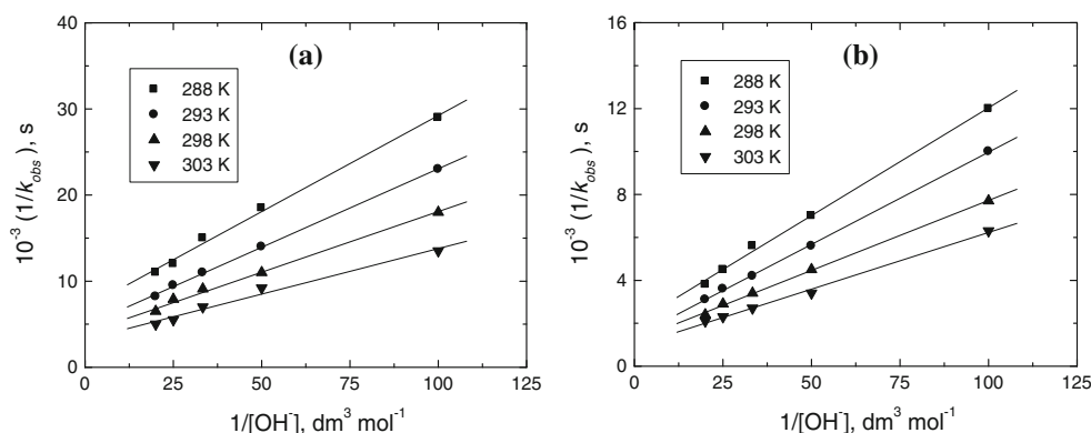
Fig. 3 a, b Plots of 1/k_{\text{obs}} versus 1/[\text{OH}^-] for the formation of the intermediate complexes in the oxidation of (a) Pym-F and (b) Py-F by alkaline permanganate at different temperatures. [\text{Azn-F}] = 8 \times 10^{-3} and [\text{MnO}_4^-] = 4 \times 10^{-4} \text{ mol dm}^{-3}
