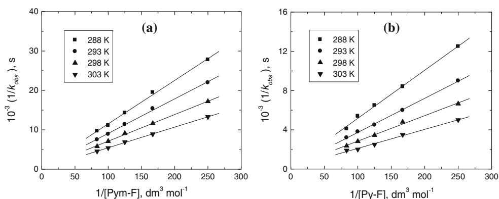
Fig. 2 a, b Double reciprocal plots for the formation of the intermediate complexes in the oxidation of (a) Pym-F and (b) Py-F by alkaline permanganate at different temperatures.
