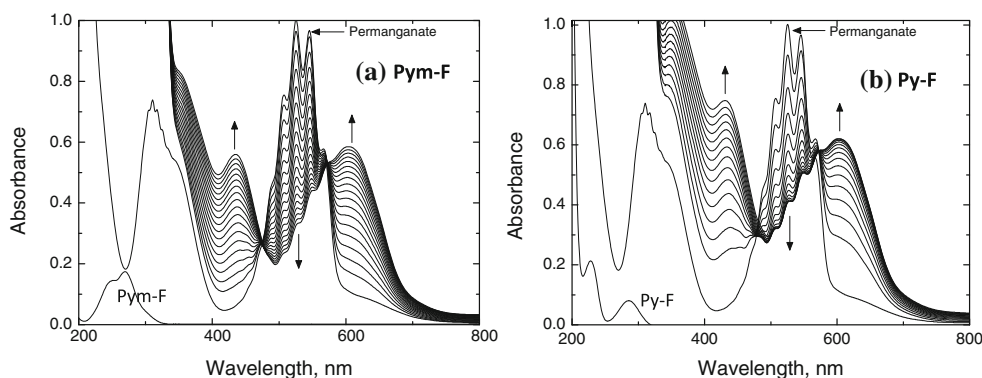
Fig. 1 a, b Spectral changes for the oxidation of azinyl formamides by alkaline permanganate.
