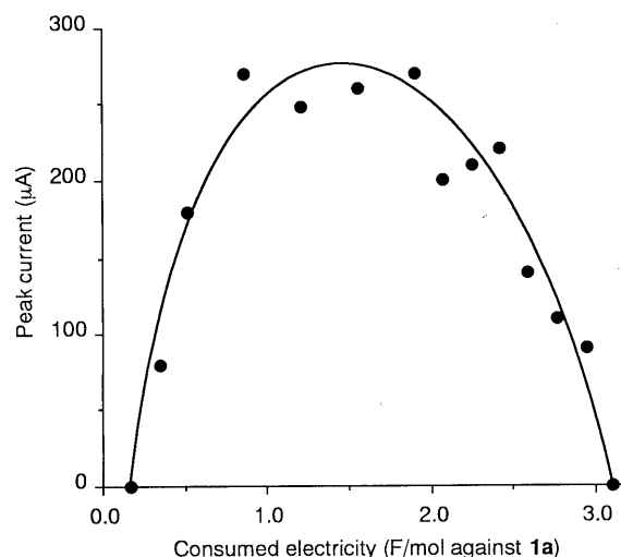
Fig. 2. Change in the Peak Current of the Voltammetric Reduction Wave Obtained during the Preparative CCE of a Solution of \text{Ph}_3\text{P} , \text{Ph}_3\text{P}^+\text{H} \cdot \text{ClO}_4^- , and 1a in \text{CH}_2\text{Cl}_2
