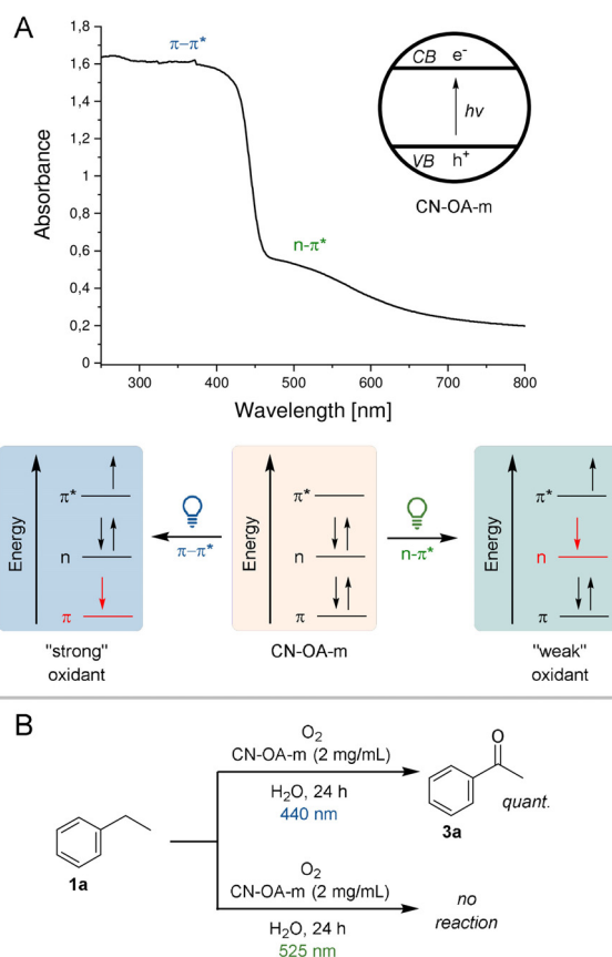
Figure 1. Chromoselective generation of excited CN-OA-m species with different oxidation potentials. A) Switching between \pi – \pi^* and n – \pi^* electron transitions using different wavelengths. B) The oxidation of ethylbenzene 1a to acetophenone 3a is only possible using blue light.
