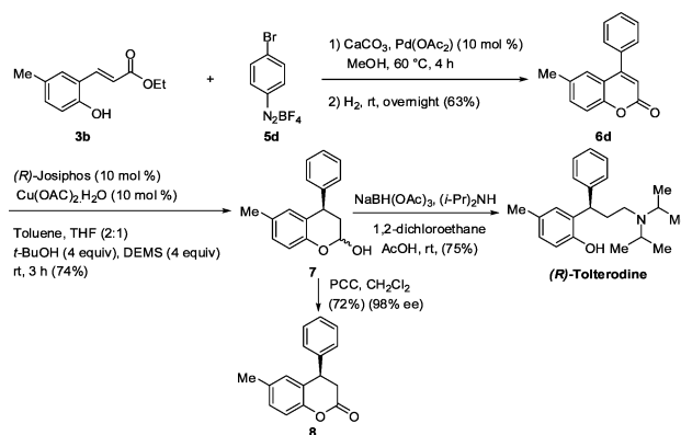
Scheme 5. Synthesis of ( R )-Tolterodine
