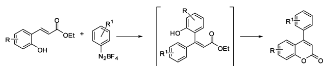
Scheme 1. Synthesis of 4-Aryl-coumarins via Tandem Heck Arylation/Cyclization
