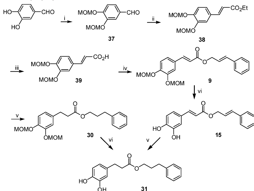
Scheme 2: Synthesis of Esters 9 , 15 , 30 , and 31 a
