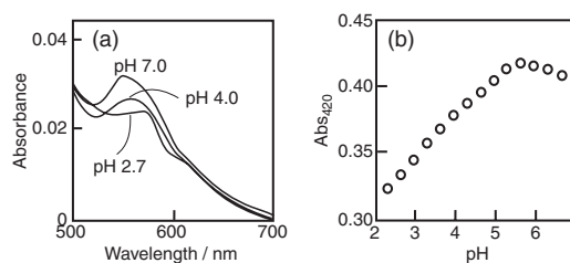
Figure 2. UV/vis spectra of 1 (3.5 \mu M) (a) at pH 7.0, 4.0, and 2.7. (b) Absorbance at 420 nm of 1 vs pH.
