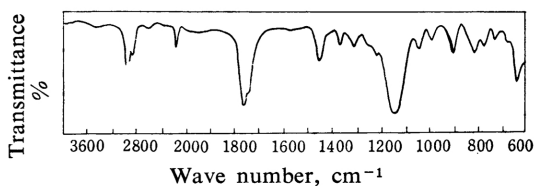
Fig. 3. Infrared spectrum of butoxycarbonylthiocyanate (IVb). (film)
