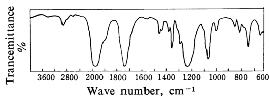
Fig. 1. Infrared spectrum of ethoxycarbonylthiocyanate (Va). (film)
