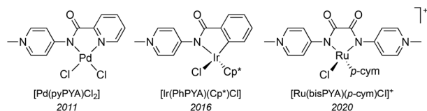
Fig. 1 Selected literature precedents of PYA complexes: [\text{Pd}(\text{pyPYA})\text{Cl}_2] ( R = \text{Me} , benzyl), [\text{Ir}(\text{PhPYA})(\text{Cp}^*)\text{L}] ( L = \text{Cl} , MeCN), and [\text{Ru}(\text{bisPYA})(p\text{-cym})\text{Cl}]^+ ( p\text{-cym} ) \text{Cl}]\text{PF}_6 .
