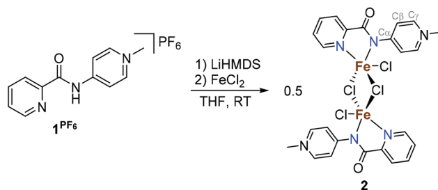
Scheme 2 Synthesis of 2 . C \alpha , C \beta and C \gamma are defined in 2 .
