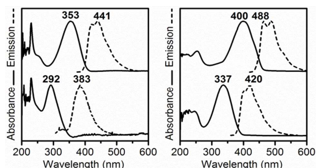
Figure 3. UV-Vis absorption and emission spectra in dichloromethane of Cp(Th) 2 (bottom left), Cp(Th 2 ) 2 (top left), Ph-Th 2 (bottom right) and DMQrT (top right).
