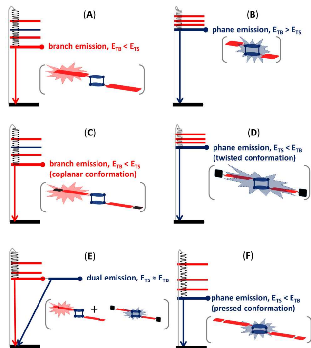
Scheme 5. Relative disposition of the relevant excited states (red: TB states on the branches; blue: TS state in the pCp unit). A) Emission from the TB state in large conjugated arms. B) Emission from the TS state in short conjugated arms. C)
