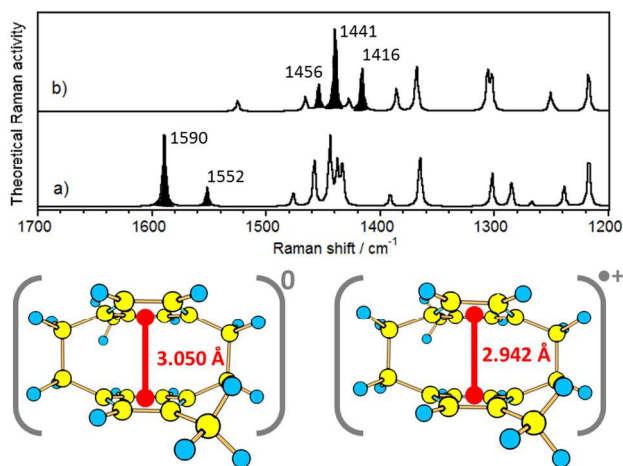
Figure 6. Top: (U)B3LYP/6-31G* theoretical Raman spectra of the dimethyl pCp unit in the neutral (a) and radical cation (b) states. Bottom: Optimized geometries with the inter-benzene average distances.
