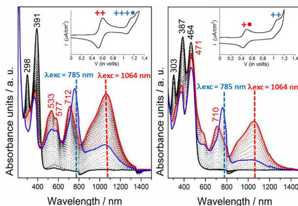
Figure 7. UV-Vis-NIR spectroelectrochemistry of Cp(PV-DA) 2 (left) and of (PV-DA) Cp(PV-DCV) (right). Dashed bars show the wavelength of the laser excitation used in the Raman experiments. The inserts correspond to the cyclic voltammetry of each compound in the anodic branch showing the formation of different polycationic states.
