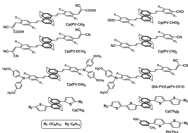
Scheme 2 Chemical structures and abbreviation of the pCp studied in this work.
