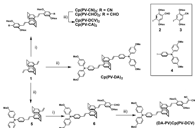
Scheme 3 Preparation of stilbene-based donor-donor, acceptor-acceptor and donor-acceptor materials. Reagents and conditions: i) Corresponding reagent 2 or 3 , Pd(OAc) 2 , Bu 4 NBr, K 2 CO 3 , DMF, 100 °C; ii) 4 , Pd(OAc) 2 , Bu 4 NBr, K 2 CO 3 , DMF, 100 °C; iii) Corresponding reagent dicyanomethane or cyanoacetic acid, AcOH, NH 4 Ac, CHCl 3 .
