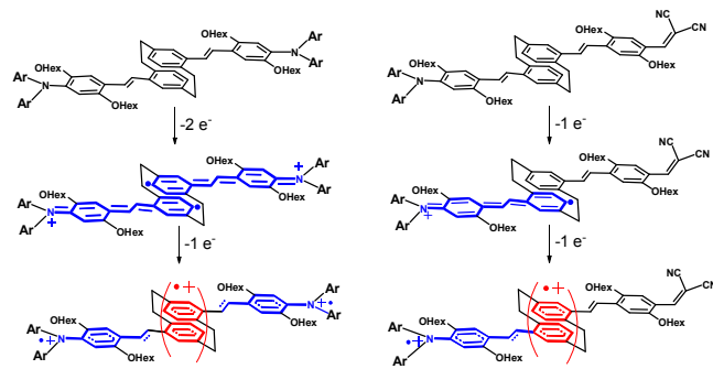
Scheme 6. Resonant forms stabilizing the charged species of \text{Cp(PV-DA)}_2 (left) and of (\text{PV-DA})\text{Cp(PV-DCV)} (right).
