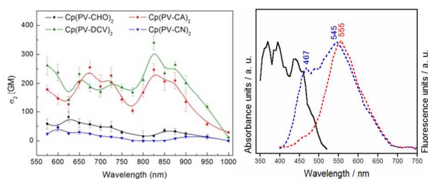
Figure 4. Left: two-photon absorption spectra recorded with the Z-scan techniques. Right: two-photon induced up-conversion fluorescence analysis for compound Cp(PV-DCV) 2 in DMF.
