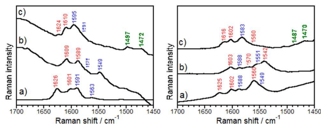
Figure 8. Left: Raman spectra of (a) neutral, (b) dication (1064 nm) and (c) radical trication (785 nm) of \text{Cp(PV-DA)}_2 . Right: Raman spectra of the (a) neutral, (b) radical cation (1064 nm) and (c) dication (785 nm) of (\text{PV-DA})\text{Cp(PV-DCV)} . In parenthesis the excitation wavelength used in the Raman experiment, (see Figure 7).
