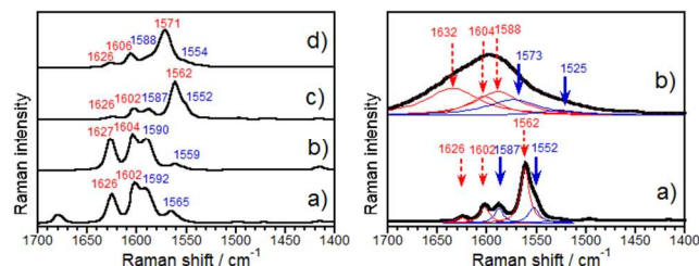
Figure 5. Left: FT-Raman spectra of the four compounds in solid state: a) Cp(PV-CHO) 2 , b) Cp(PV-CN) 2 , c) Cp(PV-DCV) 2 , d) Cp(PV-CA) 2 . Right: Raman spectra of Cp(PV-DCV) 2 in solid state at a) room pressure and b) 8 GPa. Lorentzian deconvolutions are shown in colors.
