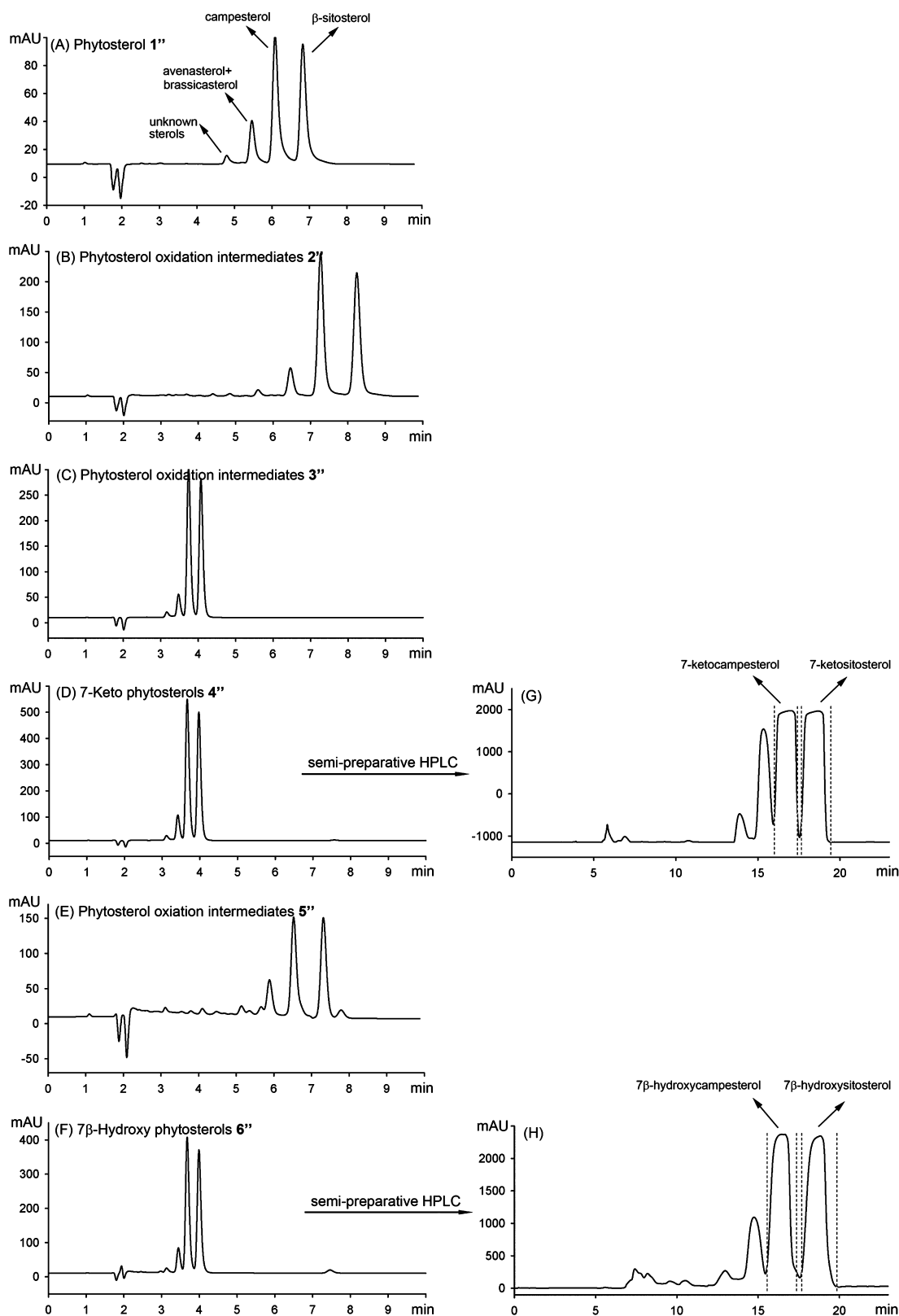
Figure 2. Analytical HPLC chromatograms of phytosterols 1'' (A), synthetic intermediates 2'', 3'', and 5'' (B, C, and E) and oxides 7-ketophytosterols 4'' (D), 7 \beta -hydroxyphytosterols 6'' (F), and semipreparative HPLC chromatograms of 4'' (G) and 6'' (H). HPLC analysis was performed on an Agilent 1200 series instrument (Santa Clara, CA, USA). Analytical HPLC conditions: Agilent Eclipse XDB-C8 column (150 \times 4.6 mm i.d., 5 \mu m); mobile phase, acetonitrile/isopropanol = 95:5 (v/v) at a flow rate of 1.0 mL/min; UV detection at 208 nm. Semipreparative HPLC conditions: Agilent Eclipse XDB-C8 column (250 \times 9.6 mm i.d., 5 \mu m); mobile phase, acetonitrile/isopropanol = 10:1 (v/v) at a flow rate of 1.5 mL/min; UV detection at 208 nm. Injection volume = 1 mL of saturated acetonitrile solution of 4'' or 6''.
