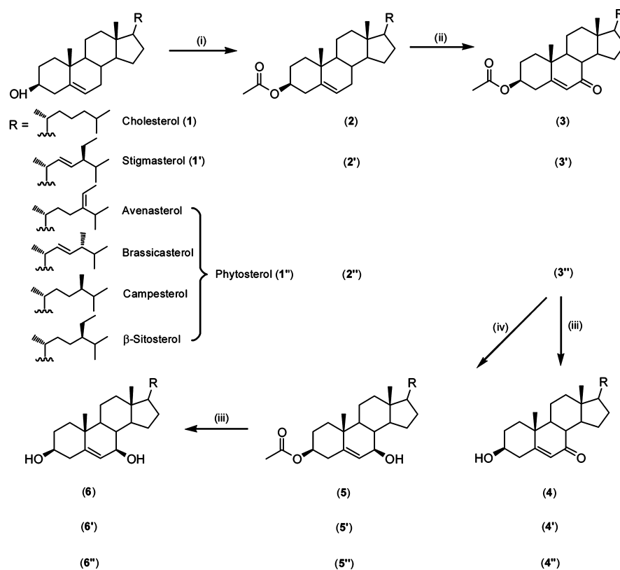
Scheme 1. Chemical Synthesis Pathway of Cholesterol Oxides (4 and 6), Stigmasterol Oxides (4' and 6'), and Phytosterol Oxides (4'' and 6'') a
