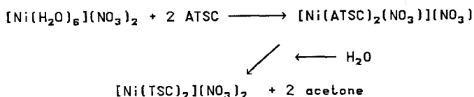
Scheme 2. Hydrolysis of the compound [Ni(ATSC)_2(NO_3)](NO_3) obtained in situ, method M2
